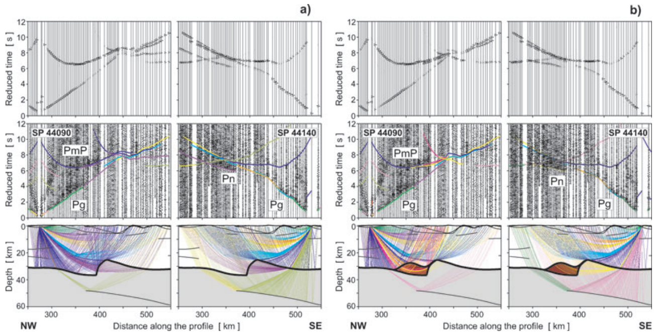
Figure 8. Forward modelling for reciprocal shot points SP 44090 and SP 44140 illustrating the character of the crust–mantle transition in the Moravo-Silesian. (a) Velocity contrast at the Moho as in Fig. 5. (b) High gradient crust–mantle transition zone according to the CEL10 interpretation (Hrubcová et al. 2008). For each part of the figure: (top panel) synthetic seismic sections, (middle panel) amplitude normalized record sections with theoretical traveltimes, (bottom panel) model and ray paths. Data have been bandpass filtered from 2 to 15 Hz. Reduction velocity is 8 \text{ km s}^{-1} . High-velocity lower crust is marked in brown.
