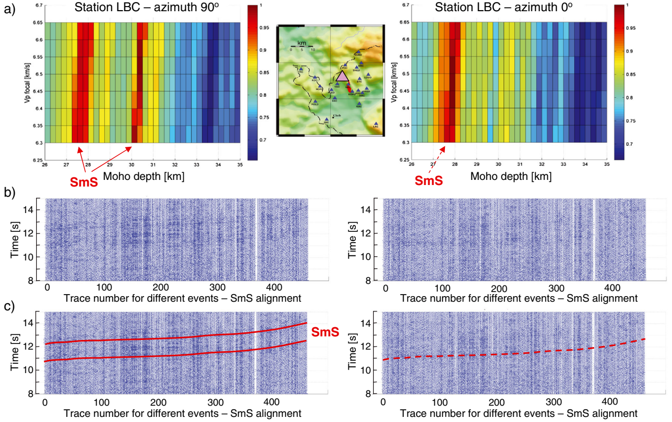
Figure 13. Inversion of the SmS reflections for the Moho depth at station LBC. The horizontal velocity records are rotated into azimuths 90^\circ (left panels) and 0^\circ (right panels). Pronounced SmS reflections from the top and bottom of the Moho zone are visible in different azimuths. (a) Stacked and inverted SmS phases with the grid search algorithm. The scale of the plot is normalized to the maximum amplitude of the stack. (b) Moho reflected SmS phases in the data. (c) Moho reflected SmS phases in the data with traveltimes calculated using ray tracing (red lines). Note optimum azimuth of 90^\circ with the most pronounced energy corresponding to the reflections at the depths of 27.50 and 30.25 km (solid red lines). The energy in the perpendicular azimuth of 0^\circ is much weaker and only detects a reflector at a depth of 27.75 km (dashed red line). Position of station LBC in the geographical map is marked by a pink triangle.
